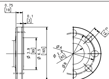
IH14 / IH17: DN50 PN25 (4 hole) \varnothing = 4.92 Inches / 125 mm 2" ANSI B16.5 Class300 (8 hole) \varnothing A = 5 Inches / 127 mm JIS B2239 2" 40K (8 hole) \varnothing B = 5.12 Inches / 130 mm
